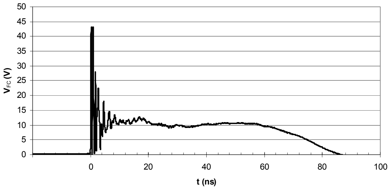
Clamping voltage at real ESD event according to IEC61000-4-2, 8 kV contact discharge
